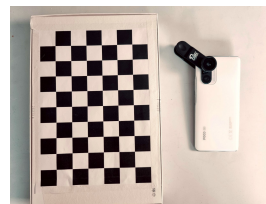
Fig. 2. Complete setup for shading estimation: a calibration pattern on the left, a smartphone with clipped-on fisheye on the right.
