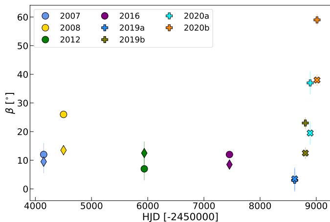
Fig. 9. Evolution of the magnetic field obliquity with respect to the stellar rotation axis. Values estimated from Eq. 3 (Stibbs 1950) using optical and near-infrared data are illustrated as circles and pluses, colour-coded by epoch, whereas values from ZDI are shown as diamonds and crosses. The y axis is expressed in degrees of colatitude.
