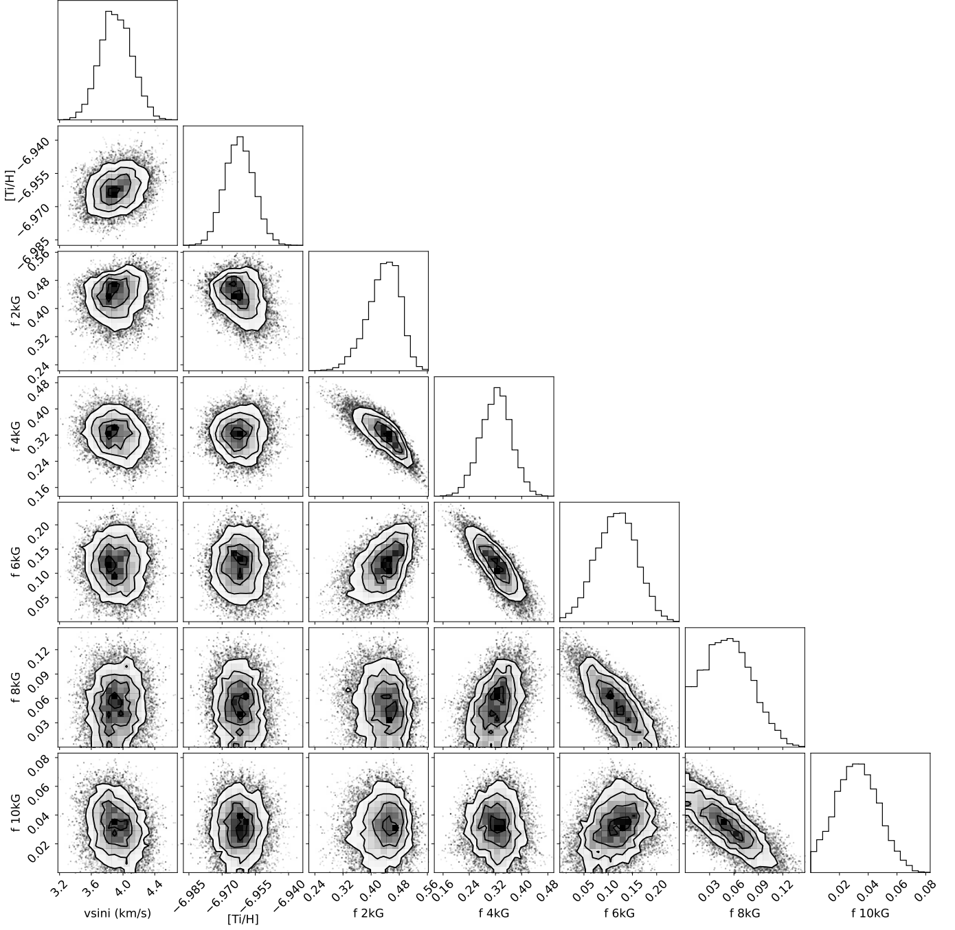
Fig. C.1. Posterior distribution for parameters from the Zeeman broadening analysis of the ESPaDOnS observation on 24 February 2016. The filling factor for a given magnetic field strength is f , and abundances are in \log n_X/n_H units.
