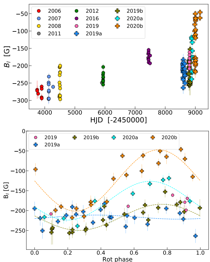
Fig. 2. Temporal evolution of the longitudinal magnetic field ( B_l ). Top: full time series of measurements between 2006 and 2020 with ESPaDOnS, Narval and SPIRou. The shape of the data points corresponds to the wavelength domain, optical (circles) or near-infrared (pluses), and the colour to the epoch in which the observations were performed. Bottom: SPIRou time series split in four epochs phase-folded according to Eq. 1. The least-square sine fit corresponding to Eq. 3 (Stibbs 1950), to assess the change in magnetic obliquity, is shown as dashed lines. The six ESPaDOnS observations taken in 2019 are plotted as pink circles.
