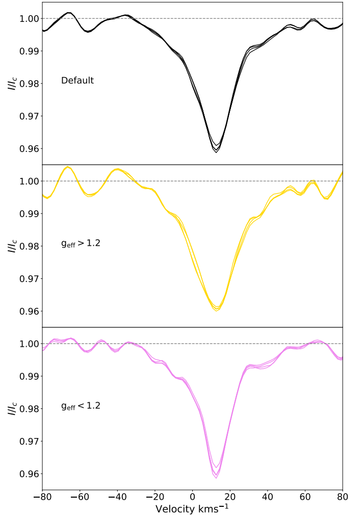
Fig. A.1. Median Stokes I profiles computed for the four near-infrared epochs: 2019a, 2019b, 2020a, and 2020b. The profiles are obtained using the full mask (top) magnetically sensitive (middle) and insensitive (bottom) line lists in LSD. Following the linear dependence of the Zeeman effect on the Landé factor, high- g_{\text{eff}} lines are broader than low- g_{\text{eff}} lines on average. The width of the profiles changes over time in the high- g_{\text{eff}} case, while it remains reasonably constant in the low- g_{\text{eff}} case.
