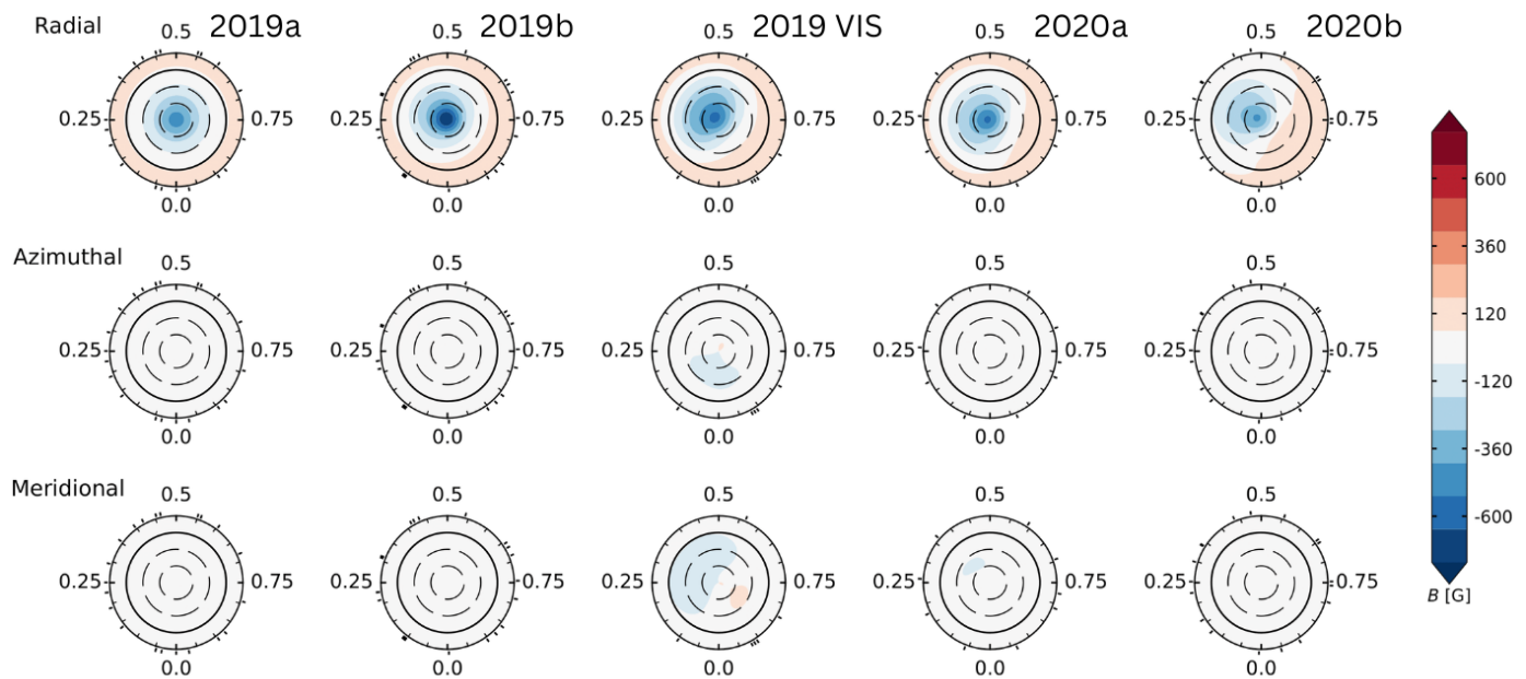
Fig. 8. Reconstructed ZDI maps in flattened polar view of AD Leo for the SPIRou and 2019 ESPaDOnS time series. The columns correspond to the epochs examined, from the left: 2019a, 2019b, 2019 optical, 2020a, and 2020b. In each column, the radial (top), azimuthal (middle) and meridional (bottom) components of the magnetic field vector are displayed. The radial ticks are located at the rotational phases when the observations were collected, while the concentric circles represent different stellar latitudes: -30^\circ , +30^\circ and +60^\circ (dashed lines) and equator (solid line). The colour bar range is set by the maximum (in absolute value) of the magnetic field and illustrates the positive (red) and negative (blue) polarity for each epoch.
