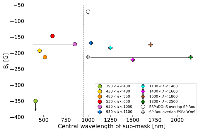
Fig. 13. Test on B_l measurements chromaticity. Shown are B_l measurements obtained with line mask subsets based on wavelength of the optical (circles) and near-infrared (pluses) domain. The horizontal black lines indicate the values of B_l computed with the full masks and the vertical dashed line separates arbitrarily optical from near-infrared measurements. The error bars are smaller than the symbol size. For visualisation purposes, the [350, 390] nm wavelength bin is not shown since it leads to an outlier data point at around -1 kG, and the [390, 430] nm bin yields a value at -750 G so it is indicated with a downward arrow. Overall, no chromatic trend emerges from the data.
