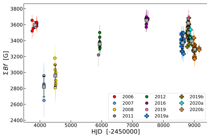
Fig. 6. Long-term evolution of the magnetic flux density measured from Zeeman broadening modelling. The data point format is the same as Fig. 2, and for each epoch we overplotted the mean value and standard deviation of B_l across both optical and near-infrared data. In addition, for the near-infrared SPIRou time series, we also observe the same oscillating behaviour found for the FWHM of Stokes I .
