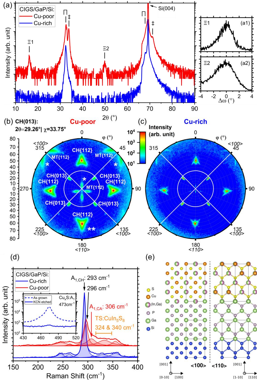
Figure 2: (a) Low resolution longitudinal \omega/2\theta scan along the [001] direction of the Si substrate. Transverse \omega scans displaying the highly textures nature of the (a1) 111 and (a2) 222 CA peaks. (bc) Pole figures of the (b) Cu-poor and (c) Cu-rich sample at the theoretical Bragg angle of the \text{CH}(013) reflection, exclusive to the CH. A white crosshair point at the predicted position of the \text{CH}(013) planes, not accounting for the 6^\circ miscut tilt. (d) Raman spectra of the Cu-rich and Cu-poor samples at 514\text{nm} excitation wavelength. Fitted peaks using Lorentzian function are drawn as a guide for the eye, and do not necessarily correspond to a specific or unique phonon mode. Inset: Zoom at the position of the
