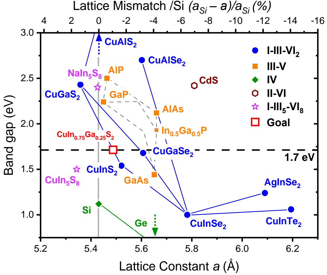
Figure 1: Band gap vs. lattice mismatch for chalcopyrites, silicon and III-V [16]. Gallium phosphide GaP is quasi lattice matched with Si. Additionally, in the Cu(In,Ga)(S,Se) 2 family, CuIn 0.75 Ga 0.25 S 2 sulfides have near ideal band gap for top cell applications. Lattice mismatch relative to a_{Si} the lattice constant of Si is represented on the top x-axis scale.
