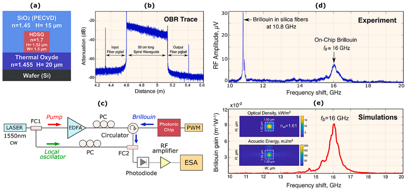
Fig. 1. (a) High-index doped silica chip waveguide cross section used for characterizing Brillouin scattering. (b) Optical backscatter reflectometer trace (spatial resolution = 20 μm). (c) Experimental setup for measuring the Brillouin backscattering spectrum. EDFA (Erbium doped fiber amplifier, PC polarization controller, FC: Fiber coupler; ESA: Electrical spectrum analyser, PWM: power meter). (d) Experimental Brillouin spectrum recorded for an input power of 18 dBm at 1550 nm, showing the Brillouin shift at 16 GHz for the high-index chip and at 10.8 GHz for the silica fibers in the setup. (e) Numerical simulation of the Brillouin gain spectrum. The insets show the computed optical (top) and acoustic (bottom) modes.
