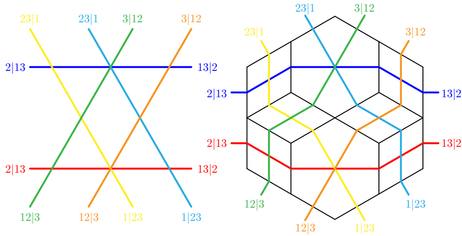
FIGURE 16. The duality between the (2,3)-braid arrangement \mathcal{B}_3^2 (left) and the diagonal of the permutahedron Perm(3) (right).
