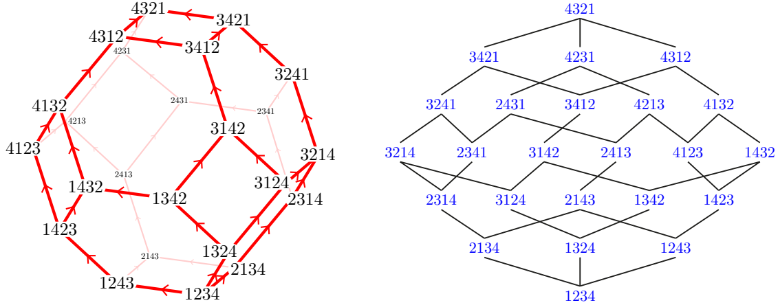
FIGURE 15. The permutahedron Perm(4) (left) and the weak order on permutations of [4] (right).
