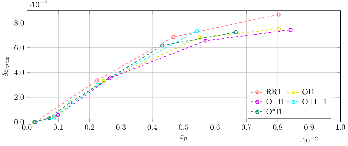
Figure 19: Evolution of the cyclic width at half-height \delta\varepsilon_{max} as a function of the strain for representative sample of each grades.
