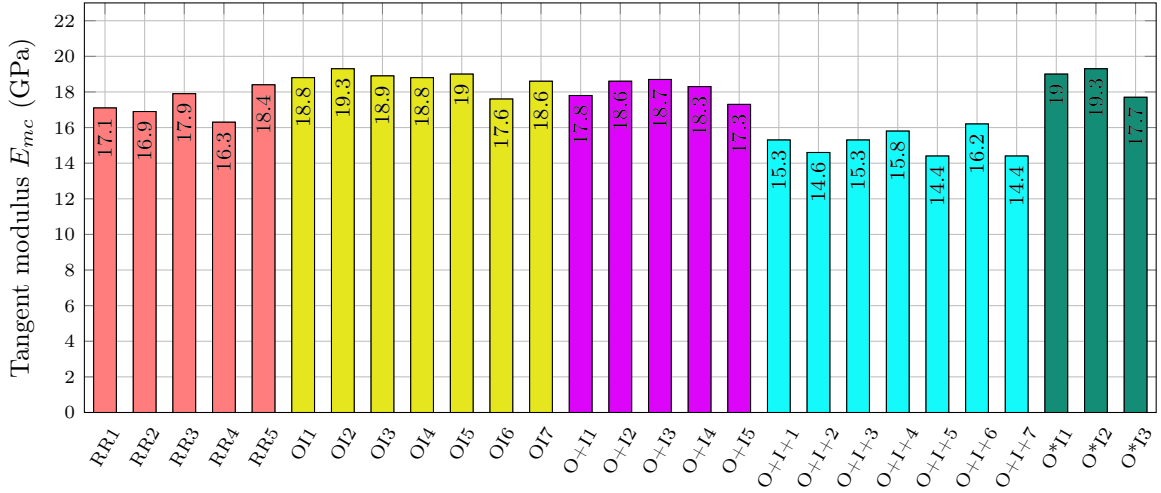
Figure 24: Tangent modulus E_{mc} for the different samples.
