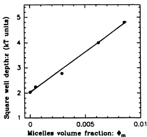
FIG. 6. Fitted square-well depth \varepsilon , in kT units, vs the micelle volume fraction \phi_m . The linear behavior is consistent with the depletion model. The extrapolation at \phi_m = 0 corresponds to an attractive background due to van der Waals attraction.
