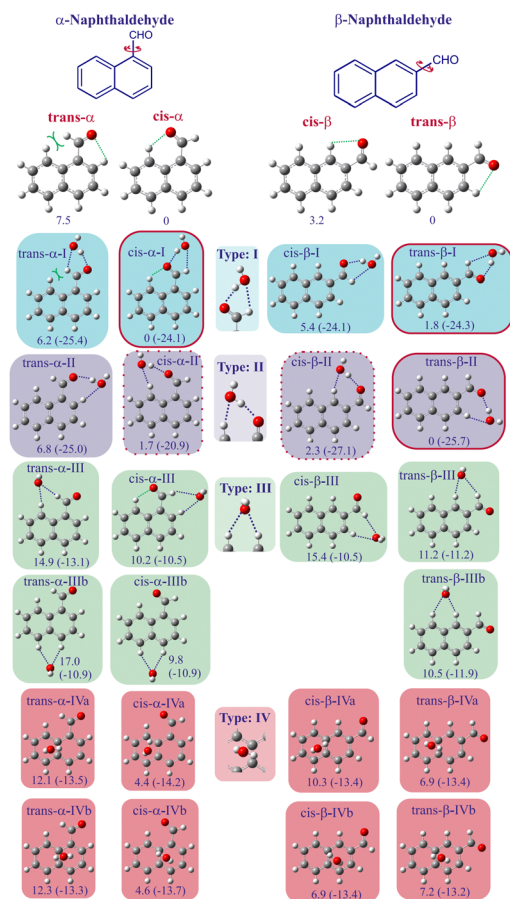
Fig. 1 Conformational landscape of the naphthaldehyde–water complexes, classified by conformation and interaction types. Structures and energies are calculated at MP2/aug-cc-pVTZ level of theory, considering ZPE correction. Relative energies are calculated between conformations with the same isomer of the naphthaldehyde subunit (12 structures at the left for \alpha and 11 structures at the right for \beta ). Values are expressed in kJ mol -1 . Values in parentheses are the hydration energies (BSSE corrected).
