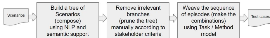
Fig. 1. Our approach in a nutshell
