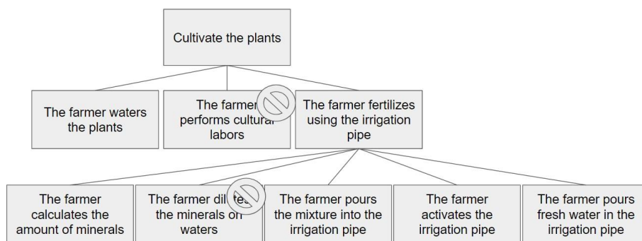
Fig. 3. Tree where manual activities are pruned
