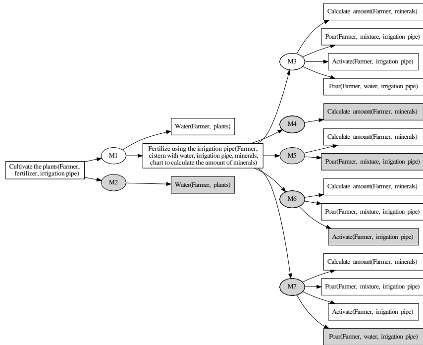
Fig. 4. Execution tree for “Cultivate the plants” task
