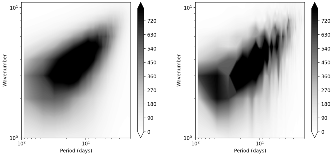
Figure 1a. H_E(k, \omega) , th = \infty .
