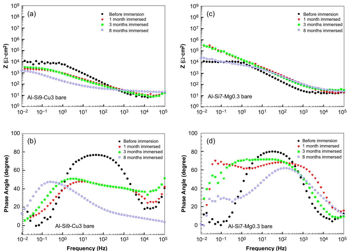
FIGURE 20. Bode plots of (a, c) impedance magnitude and (b, d) phase angle as a function of frequency recorded in artificial seawater for (a, b) Al-Si9-Cu3 and (c, d) Al-Si7-Mg0.3 samples before immersion in the Adriatic Sea and after 1, 3, and 8 months immersion. Before electrochemical measurements, the samples were sonicated to remove the biofilm formed during immersion. For the samples immersed for 8 months, it was difficult to find an area free of biofouling sufficient to perform three replicates; blue circles presented these curves.
