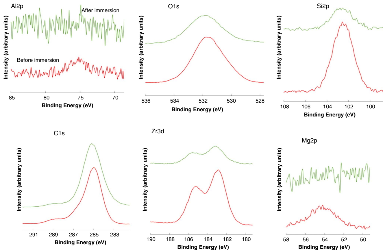
FIGURE 11. XPS high-resolution spectra recorded at the surface of Al-Si7-Mg0.3 sample coated with ZG coating before and after immersion for 1 month in the Adriatic Sea. Related survey spectra are presented in Figure S11, and the composition is in Table 4. The samples were sonicated before the analysis.
