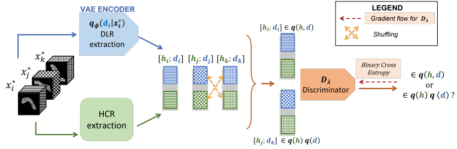
Fig. 4. Training D_\lambda . Given three different input images x_i^* , x_j^* and x_k^* , the corresponding HCR and DLR features are computed: h_j , h_j , h_k and d_i , d_j , d_k . Samples from q(h, d) are obtained by concatenating features of a same image ( h_i and d_i for instance), while samples from q(h)q(d) are obtained by concatenating h_k and d_j with k \neq j .
