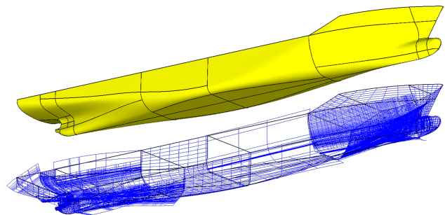
Figure 1: Top: Shaded MCAD B-rep faces of the KCS ship hull model, with edges shown in black wireframe. Bottom: Embedding NURBS patches for each face.
