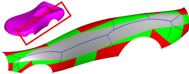
Figure 5: SubD layering for the wheel arch of the Car model, showing corner (red), edge (green) and unstructured regions (grey). The 2D medial axis (blue) determines the shape of the blocks so that they do not intersect.
