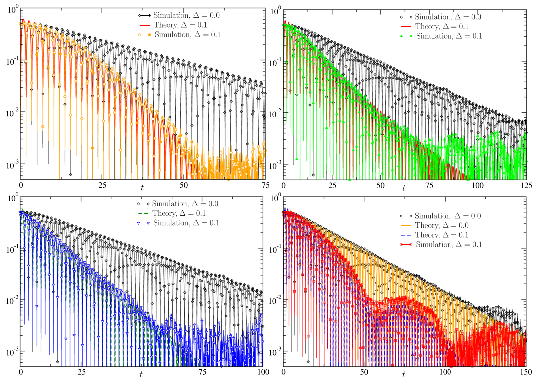
Figure 4. Time evolution of the energy consumption to its equilibrium value |N_i(t) - 1/2| is shown. Four subfigures correspond to the four different DPD cases: Gaussian (top left), Laplacian (top right), Lorentzian (bottom left), and uniform finite-support (bottom right), described by Eqs (7), (8), (9) and (10), respectively. Particle simulations are compared with analytic predictions, with the latter limited to accounting only for the two dominant modes corresponding to \lambda_{0,-} , \lambda_{-1,-} . Parameters chosen for the illustration are r = 10 , \tau_0 = 3 , -x_{\downarrow} = x_{\uparrow} = 1 , and N = 10^5 . Two different levels of the disorder, with \Delta = 0 and 0.1 , are shown in each subfigure.
