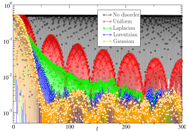
Figure 1. Results of particle simulations providing a representative comparison of the four types of disorder. We chose here the most dramatic case with almost no (additional) control by the aggregator where in the case of no disorder (all consumers are the same) the system does not mix. Introduction of disorder (diversity in the aggregator’s portfolio) results in the decay, which is most impressive in the case of the Gaussian disorder, still fast (exponential) in the case of the Lorentzian disorder, and much slower (but still noticeable, 1/t^2 and 1/t ) in the case of the Laplacian and uniform finite-support disorder. We show here |N_i(t) - 1/2| vs time, and the model parameters chosen for the comparative illustration are \tau_0 = 3, r = 100, \Delta = 0.1, -x_{\downarrow} = x_{\uparrow} = 1 , and N = 10^5 . (See “Particle Simulations and Comparison with the Theory” section for more details, e.g., for comparison of theory and simulations).
