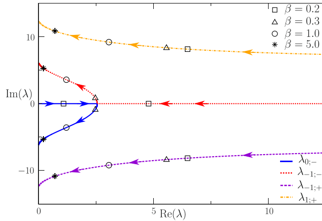
Figure 3. Evolution with increase in \beta \doteq r\tau/4 at the fixed \tau = 1 of the four leading eigenvalues, \lambda_{k;\pm}(\beta) (i.e., eigenvalues with the largest non-zero real value) is shown in the \text{Re}(\lambda_{k;\pm}(\beta))\text{-Im}(\lambda_{k;\pm}(\beta)) plane. Markers indicate \beta = 0.2, 0.3, 1, 5 . At \beta > \beta_c \simeq 0.278 , \lambda_{0;-} and \lambda_{-1;-} become complex (the eigenvalues are real otherwise) and complex conjugate. The real part of \lambda_{\pm 1;\pm} is always larger than that of \lambda_{0;-} and \lambda_{-1;-} .
