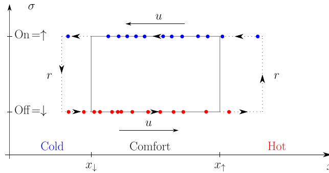
Figure 2. Schematic illustration of an instantaneous device distribution and dynamics in the (x, \sigma) phase space, where x is the (continuous) temperature, and the discrete (two-level) designation, \sigma , marks whether the device (air conditioner) is switched on, \sigma = \uparrow , or off, \sigma = \downarrow .
