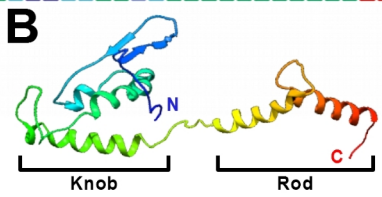
Figure 1: Structure prediction of P2. (A) Secondary structure prediction discerns between \beta -strands, \alpha -helices and disordered regions. The confidence of the prediction is indicated for each amino acid. The blue boxes show the position of the alanine substitution. (B) Three-dimensional model of P2. The colors represent the order of the amino acids from the N-terminus (dark blue) to the C-terminus (red). The overall structures suggests an N-terminal knob, separated by an unstructured stretch from a rod-like C-terminus. All predictions were made with the PHYRE2 program 40 .
