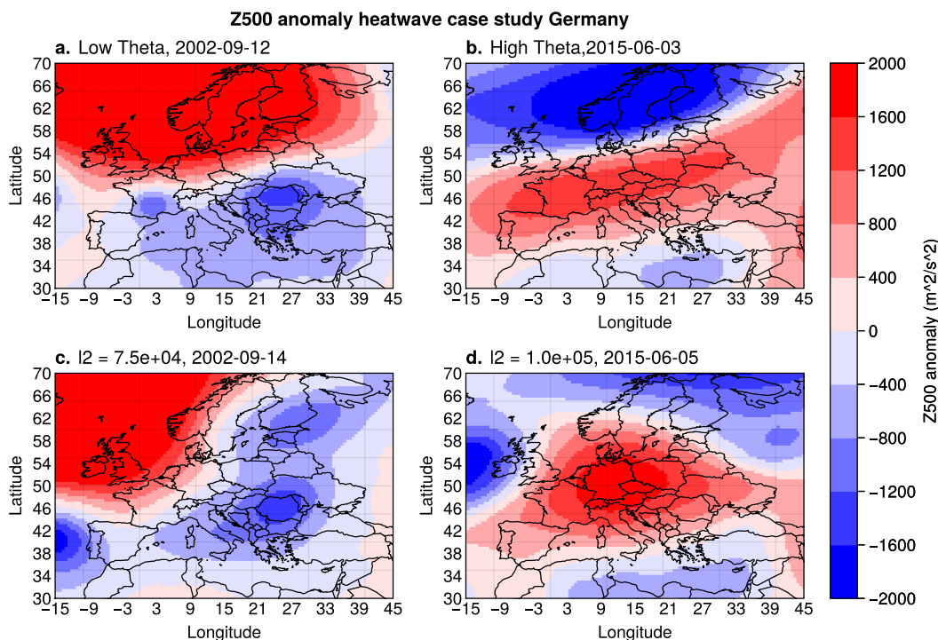
Figure 6. Z500 maps corresponding to the days with the highest and lowest \theta within all days which are classified as days where there is a heatwave in the region Germany. Panel titles in (c), (d) show a lead time of 2 days to the respective high and low \theta heatwave days, with the values corresponding to the euclidean distance between the initial and 2 day lead SLP maps for each case.
