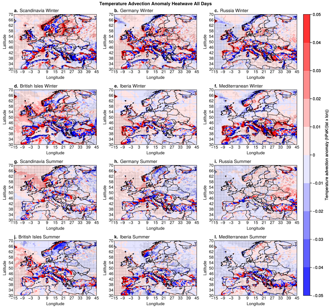
Figure 4. B [ \text{hPaK}/\text{lat} \times \text{lon} ] composite anomaly, corresponding to surface temperature advection, during warm spell and heatwave days in (a, g) Scandinavia, (b, h) Germany, (c, i) Russia, (d, j) British Isles, (e, k) Iberia, (f, l) Mediterranean, during winter (a–f) and summer (g–l). Positive anomalies, denoted by the colour red, represent warm advection, whilst the colour blue corresponds to cold air advection. Statistical significance is denoted with grey stippling and assessed as described in Section 2.
