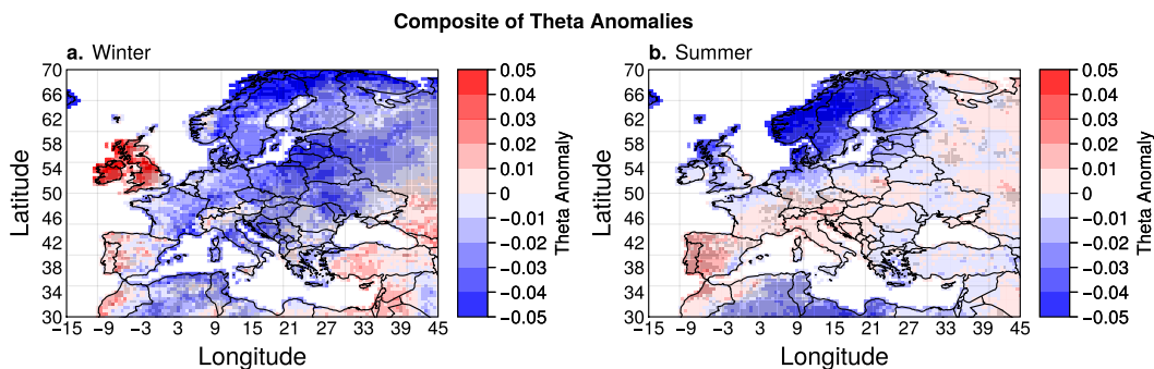
Figure 2. \theta [1/days] anomalies for all warm spell or heatwave days for each grid box, during winter (a) and summer (b). Statistical significance is assessed as described in Section 2 and shown with grey stippling.
