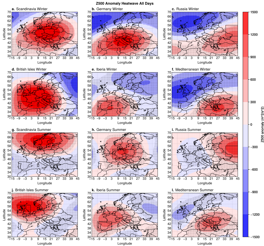
Figure 1. Composite Z500 [ \text{m}^2/\text{s}^2 ] anomalies during warm spell/ heatwave days in (a,g) Scandinavia, (b, h) Germany, (c, i) Russia, (d, j) British Isles, (e, k) Iberia, (f, l) Mediterranean, during winter (a–f) and summer (g–l). Statistical significance is assessed as described in Section 2 and shown with grey stippling.
