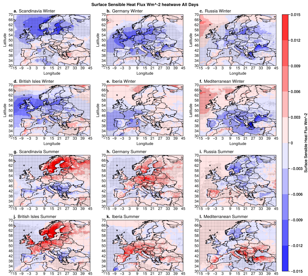
Figure 5. SSHF [ \text{W}/\text{m}^2 ] composite anomalies during warm spell and heatwave days in (a, g) Scandinavia, (b, h) Germany, (c, i) Russia, (d, j) British Isles, (e, k) Iberia, (f, l) Mediterranean, during winter (a-f) and summer (g-l). Statistical significance is denoted with grey stippling and assessed as described in Section 2.
