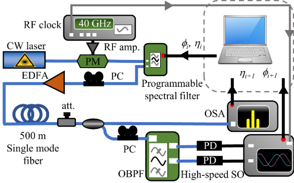
Fig. 1 Experimental setup. PC – polarization controller, Att. – attenuator, OBPF – optical band pass filter, PD – photodiode, RF amp. – radiofrequency amplifier.
