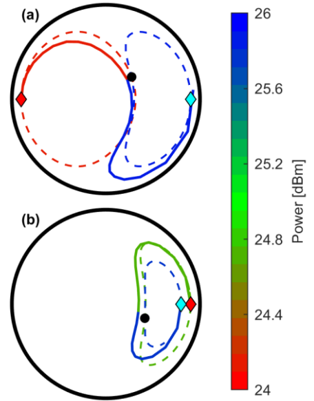
Fig. 2 Experimental trajectories that connect (a) \eta_{IN} = 0.90 , \phi_{IN} = \pi and \eta_{OUT} = 0.90 , \phi_{OUT} = 0 , (b) \eta_{IN} = 0.90 , \phi_{IN} = 0 and \eta_{OUT} = 0.80 , \phi_{OUT} = 0 , by an abrupt power change. The colour depicts value of input average power that is used for each part of the trajectory.
