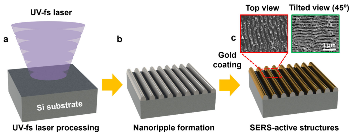
Figure 1. Preparation of UV-fs-laser-textured Si substrates with 34 nm Au coatings. (a) UV-fs laser processing by changing hatching distances and laser fluences (Wavelength: 343 nm; pulse duration: 400 fs; pulse energy 48.3 μJ); (b) Formation of nanoripples on Si substrates; and (c) Au-coated Si substrates with nanoripples.
