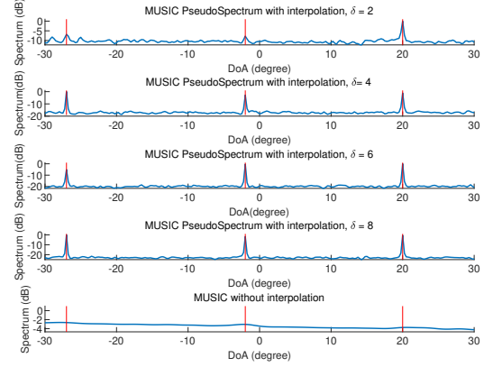
FIGURE 3. MUSIC Pseudo-spectrum versus \theta with three coherent signals from directions -27^\circ, -2^\circ, 20^\circ , \theta_{B,k} = \theta_k , and \text{SNR} = 7\text{dB} .
