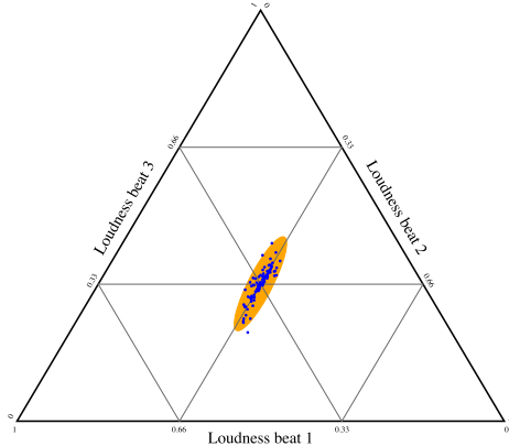
(a) Small area of the ellipse in the loudness simplex from Kapell's interpretation of Mazurka 6-2 indicating an interpretation with regular loudness.
