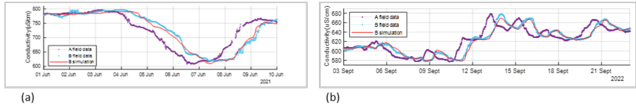
Figure 3. Measured conductivity at point A (upstream, purple) and measured (blue) and simulated (red) conductivity at point B (downstream), in June 2021 (a) and September 2022 (b).
