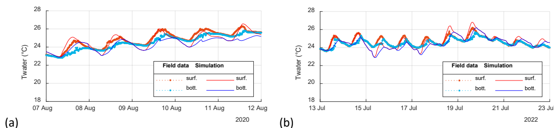
Figure 2. Measured (dotted) and simulated (line) water temperature in August 2020 (a) and July 2022 (b) at point B In the episode of conductivity variation, in June 2021, conductivity decreased from around 800 to 600 \mu\text{S}/\text{cm} in
