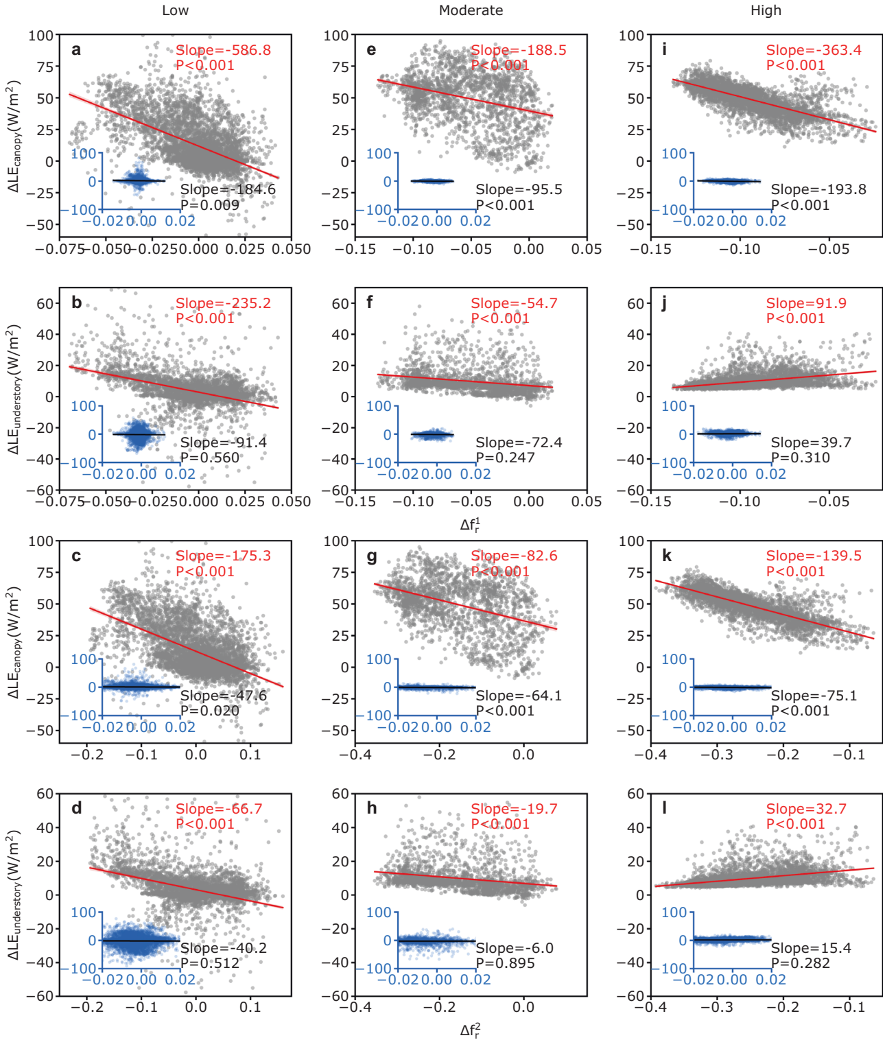
Fig. 4 Correlations of \Delta f_r^1 and \Delta f_r^2 with the components of \Delta LE ( \Delta LE_{canopy} , \Delta LE_{understory} ). The graphs a–i show the correlations of seasonal variations, while the inserts in a–i represent the correlations in the long-term variations. P -values were determined by a two-sided Student’s t -test.
