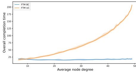
Fig. 4: Overall completion time - 50 nodes random graphs, min-max values
