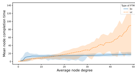
Fig. 6: Mean node completion time - 50 nodes random graphs, min-max values
