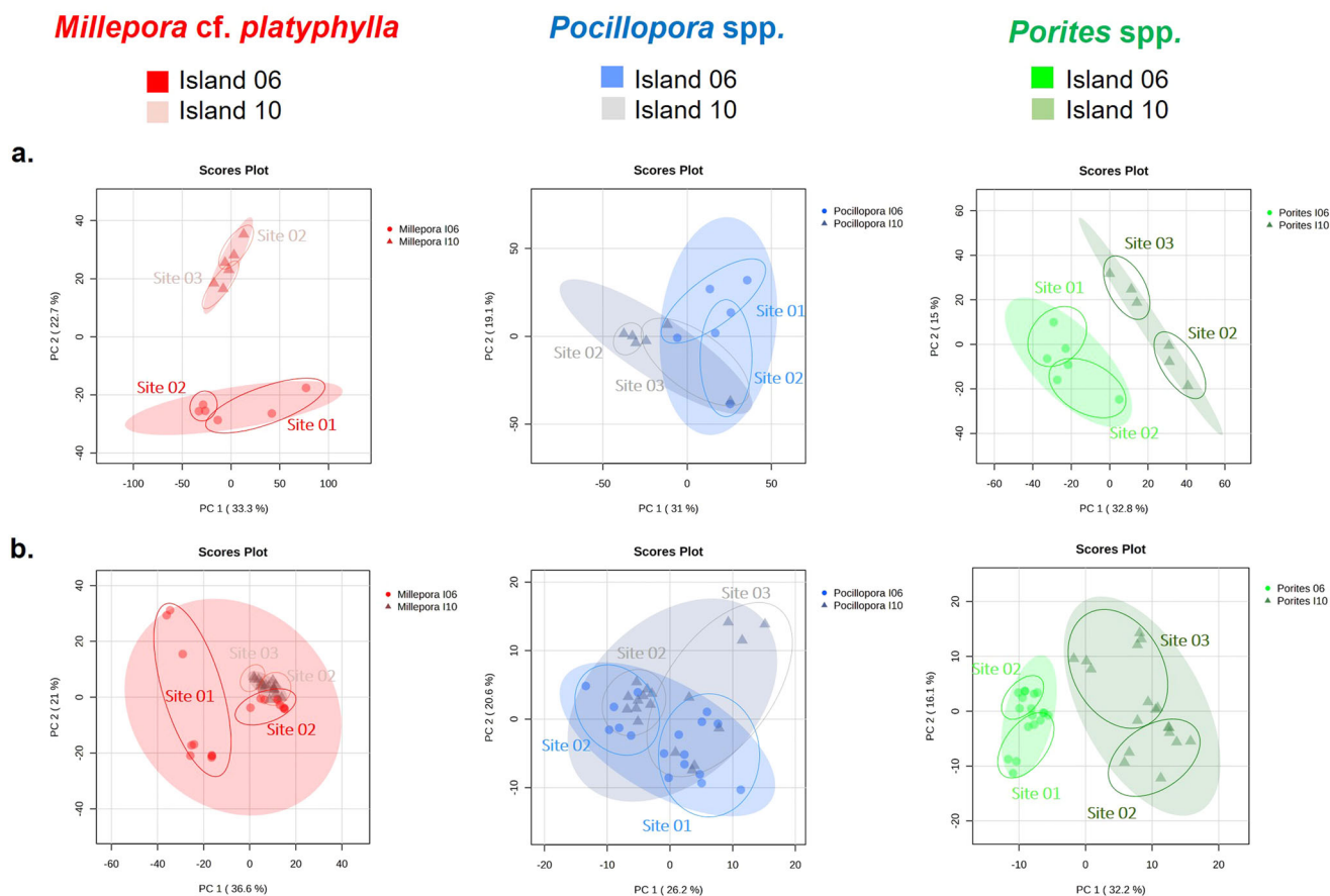
Fig. 2 Metabolome variability with geography. PCA score plots for the three host genera located in sites 01 and 02 of island 06 (Gambier) and sites 02 and 03 of island 10 (Samoa) from (a) LC-MS/MS (ESI + ), and (b) 1 H NMR.
