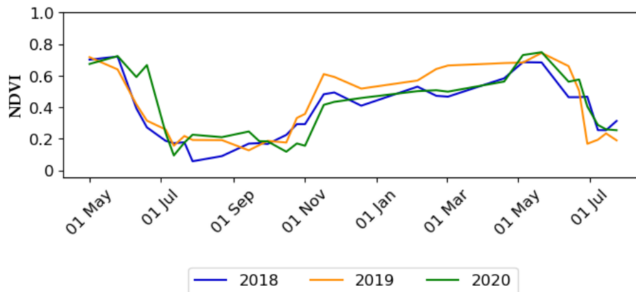
Fig. 5. NDVI temporal behavior over rapeseed fields in 2018, 2019, and 2020. The NDVI-values were calculated from Sentinel-2 images (S2), downloaded from the Theia website ( https://www.theia-land.fr/ ).
