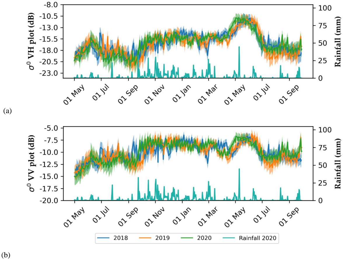
Fig. 4. Sentinel-1 temporal behavior over rapeseed fields in 2018, 2019, and 2020. (a) VH at the plot scale (VHp), (b) VV at the plot scale (VVp), The mean values are represented by bold lines and the standard deviation by the shaded areas. The rainfall events in the cultivation period of rapeseed in 2020 is presented using the secondary Y-axis.
