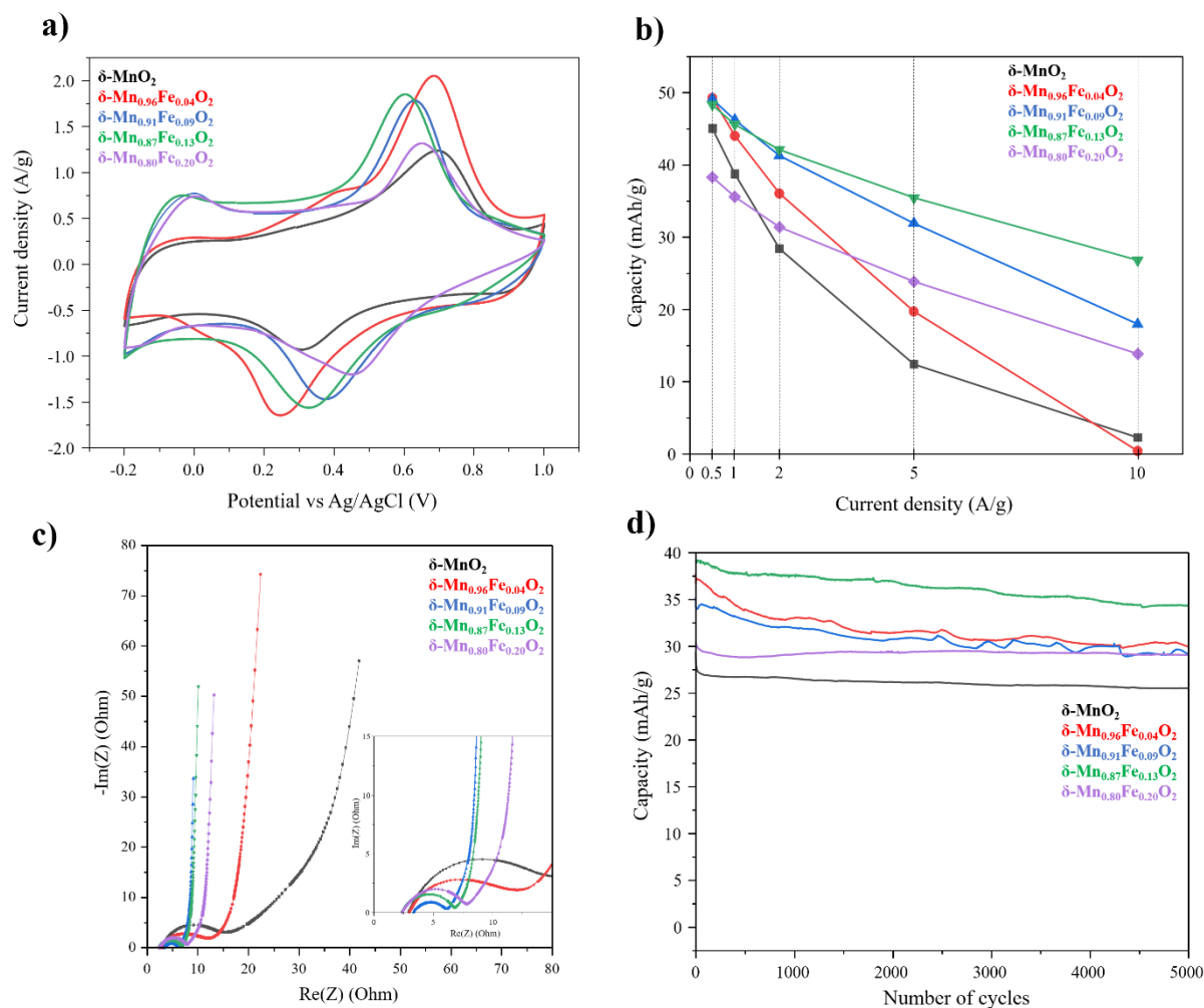
Figure 6: a) Cyclic voltammety of the synthesized birnessites at 5 mV/s in 0.5M \text{K}_2\text{SO}_4 , b) Discharge capacity retention at various current densities, c) Nyquist plots obtained from EIS measurements at open circuit potential d) Capacity evolution of the series of birnessite materials upon long term cycling in 0.5M \text{K}_2\text{SO}_4 at 3 A/g.
