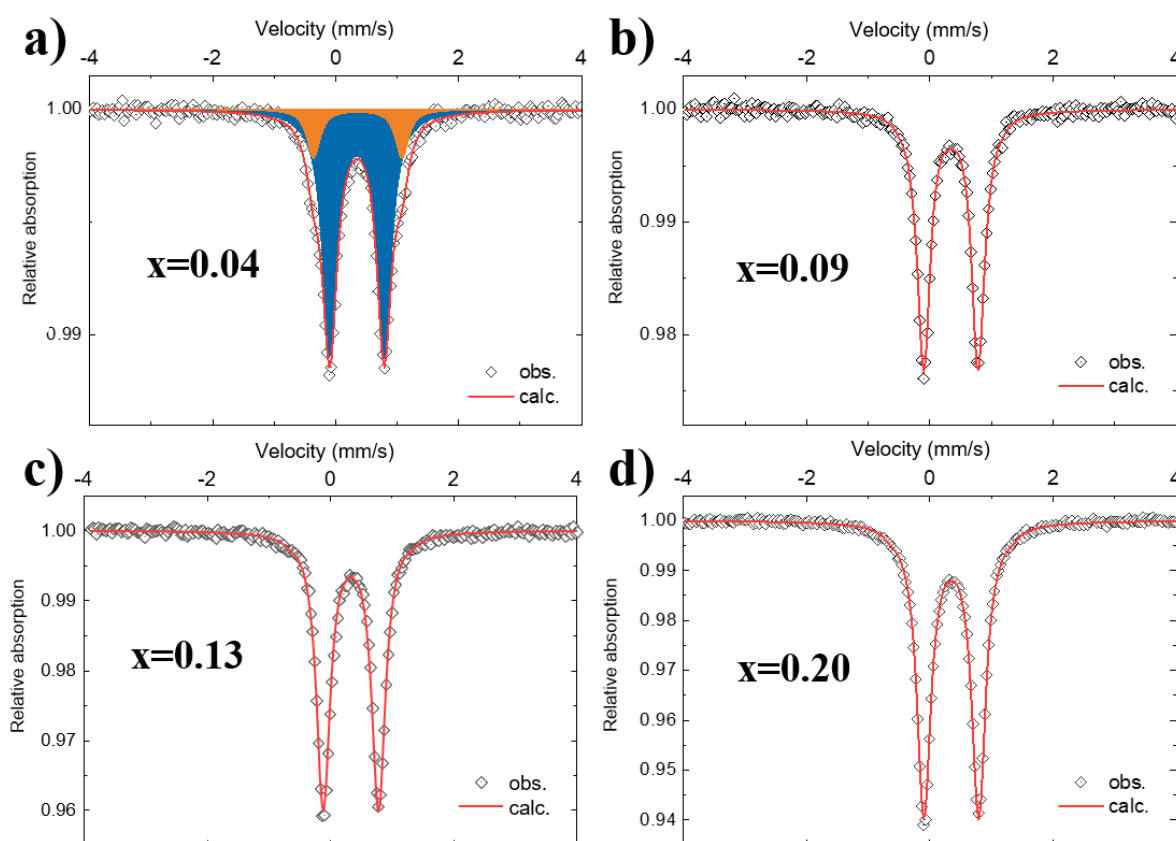
Figure 4: ^{57}\text{Fe} Mössbauer spectra at room temperature ( 25^\circ\text{C} ) of \delta\text{-Mn}_{1-x}\text{Fe}_x\text{O}_2 , a) x=0.04 , b) x=0.09 , c) x=0.13 and d) x=0.20 .
