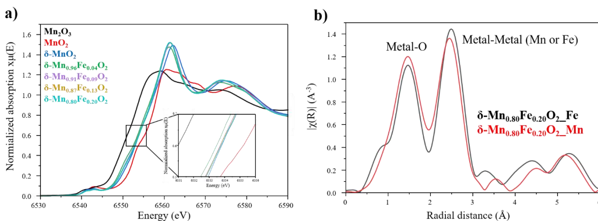
Figure 5: a) Mn K-edge XANES spectra for all the series. Mn_2O_3 and MnO_2 were used as reference to get the energy edge for Mn^{3+} and Mn^{4+} respectively. b) FT-EXAFS spectra of \delta-Mn_{0.80}Fe_{0.20}O_2 of the first iron (black) and manganese (red) neighbors.
