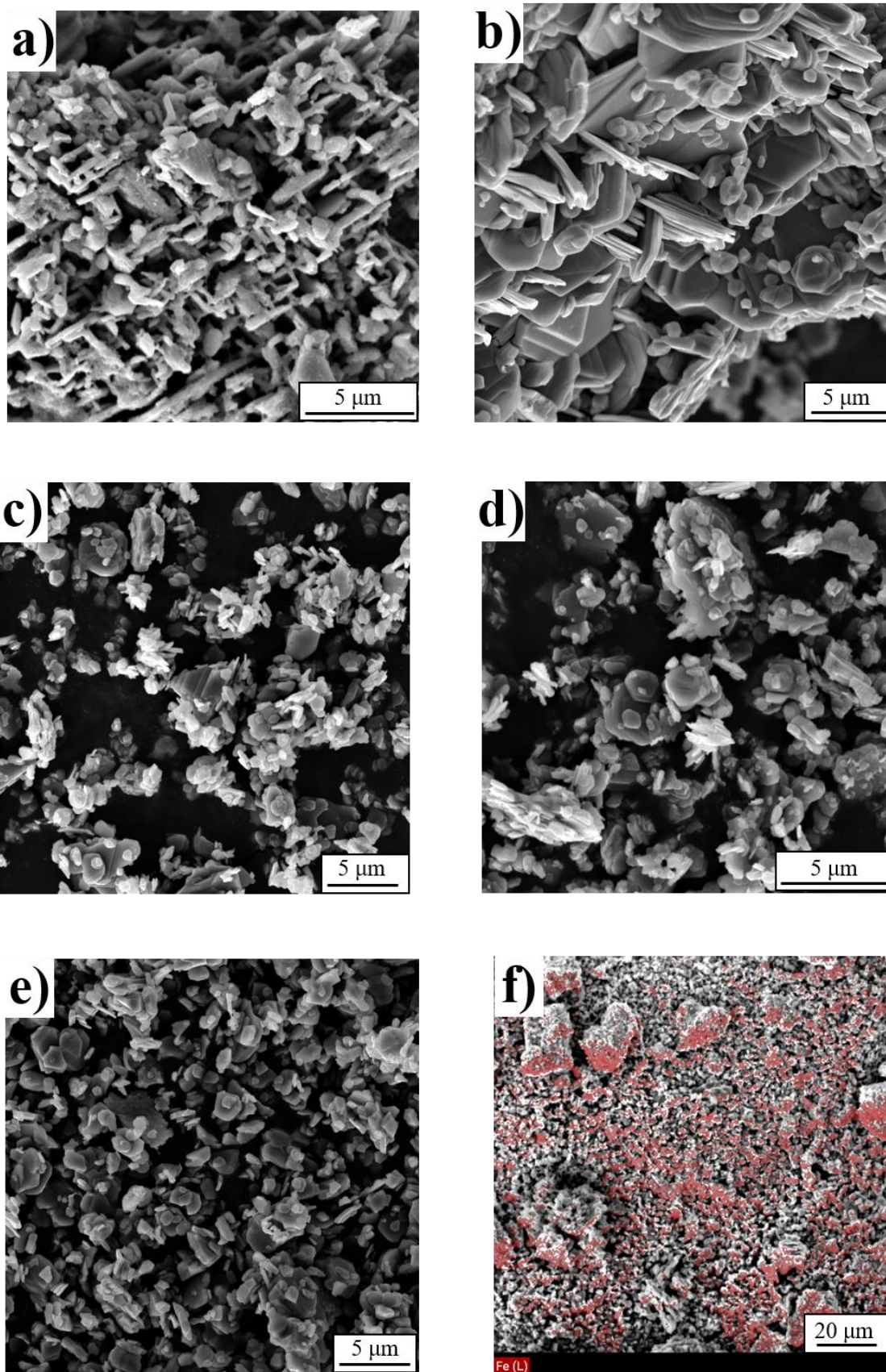
Figure 3: SEM images of a) \delta\text{-MnO}_2 , b) \delta\text{-Mn}_{0.96}\text{Fe}_{0.04}\text{O}_2 , c) \delta\text{-Mn}_{0.91}\text{Fe}_{0.09}\text{O}_2 , d) \delta\text{-Mn}_{0.87}\text{Fe}_{0.13}\text{O}_2 , e) \delta\text{-Mn}_{0.80}\text{Fe}_{0.20}\text{O}_2 and f) mapping of Fe element in \delta\text{-Mn}_{0.80}\text{Fe}_{0.20}\text{O}_2 sample.
