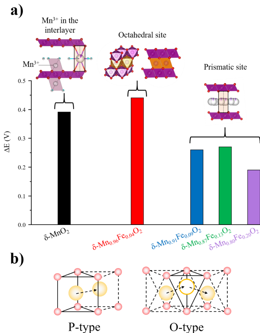
Figure 7: a) Comparison of the potential difference between the maximum of oxidation and reduction peaks extracted from the CV performed at 5 mV/s in 0.5M K 2 SO 4 b) The direct alkaline diffusion path through face sharing prismatic site in P-type frameworks and indirect alkaline diffusion path with the intermediate tetrahedron site in O-type frameworks.
