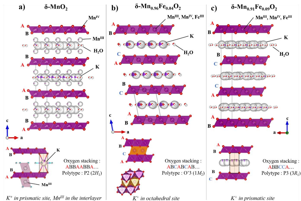
Figure 2: Crystal structures of \delta\text{-Mn}_{1-x}\text{Fe}_x\text{O}_2 , x = 0 (a), 0.04 (b), and 0.09 (c).
