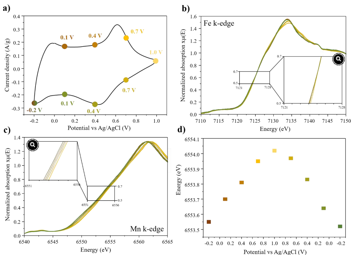
Figure 8: Cyclic voltammetry at 2 mV/s in 0.5M \text{K}_2\text{SO}_4 , b) Fe K-edge XAS spectra at different potential (refer on the cyclic voltammetry), c) Mn K-edge XAS spectra at different potentials and d) Change in shift energy as a function of the potential for \delta\text{-Mn}_{0.80}\text{Fe}_{0.20}\text{O}_2 .
