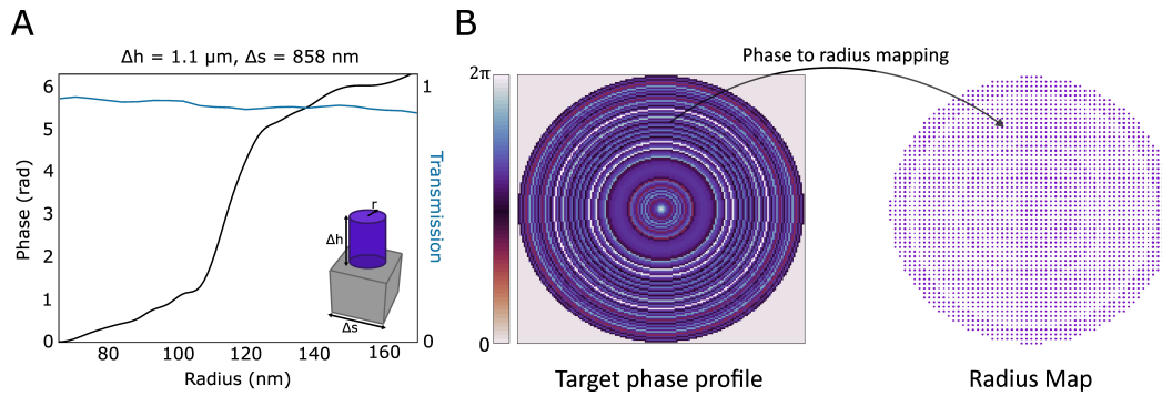
Fig. 3: Design and simulation of imaging metalenses. The metalenses are made up of GaN nanopillars with a refractive index of 2.42, where the thickness ( \Delta h ), sampling ( \Delta s ), and radius ( \Delta r ) are the design parameters. (a) Simulation of the nanopillars’ transmission amplitude and phase response via FDTD. (b) Illustration of the full metalens design, transforming the spatial phase profile into a spatial radius (of nanopillar) distribution with respect to the target phase.
