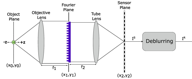
Fig. 1: A 4f system computational EDOF microscope model that combines the optical module, sensor, and D-CNN.
