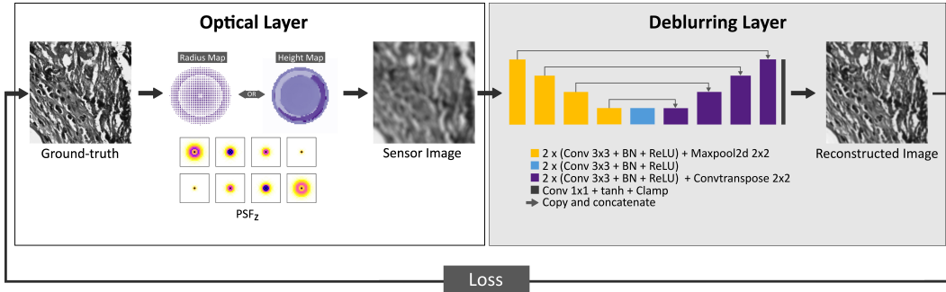
Fig. 2: Overall representation of the end-to-end framework for joint optimization of the phase coding mask and the D-CNN. The end-to-end framework consists of an optical layer that simulates image formation for the learned optics, and the deblurring layer employs U-Net architecture to reconstruct in-focus images within the desired DOF range.
