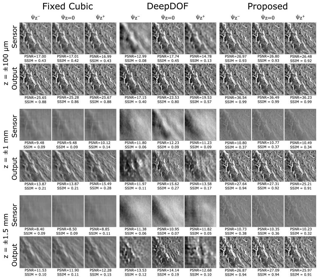
Fig. 4: Simulated performance of a cubic-mask-enabled computational 4f system, DeepDOF model, computational EDOF microscope, optimized for various target depths. For all DOFs, our method shows superior performance.
