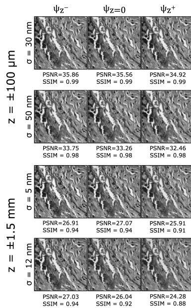
Fig. 6: Reconstruction results for increasing radius and height-map fabrication error levels.
