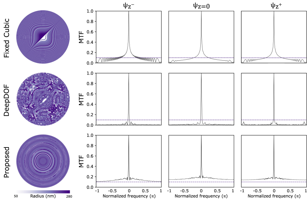
Fig. 5: The optimized metalens radius maps, as well as the MTFs at three distinct depths, are presented for the existing and proposed methods, encompassing the maximum defocus values within the 3 mm DOF scene and the in-focus depth.
