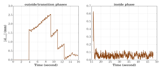
Fig. 20. The RCM task error d_{rcm} , where the left column shows the error evolution during the outside/transition phases while the right column presents the error during the inside phase.
