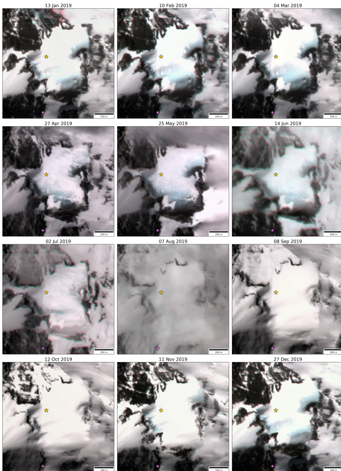
Figure 2. Natural color composites (bands 7–4–3) of VENμS images (CC BY-NC 4.0) showing the seasonal variability in the surface snow cover of South Col Glacier. The yellow star shows the location of the drilling site and the purple one the location of the South Col AWS. Note the striking expansion of blue-ice areas outside the monsoon months, i.e., January–April 2019 and October–December 2019.
