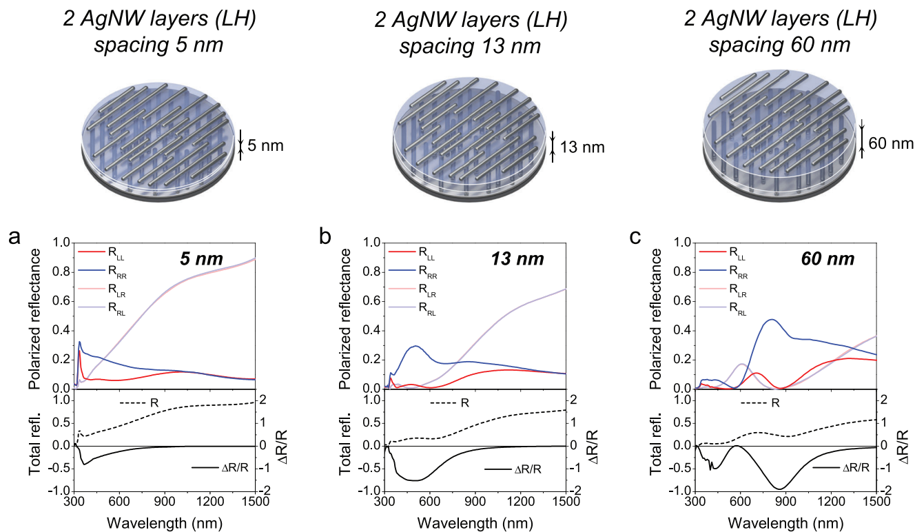
Figure 3. Spectra of the measured reflectance R labeled as function of the incoming and outgoing polarization states R_{i\sigma} and of the total reflectance R and the differential reflectance \frac{\Delta R}{R} for samples consisting of two layers of AgNWs oriented at +45^\circ (left-handed structure) deposited on top of silver mirror. The spacing between the AgNW layers is equal to a) 5 nm, b) 13 nm, and c) 60 nm. Note that the sample in (b) is the same as the one of Figure 2b.
