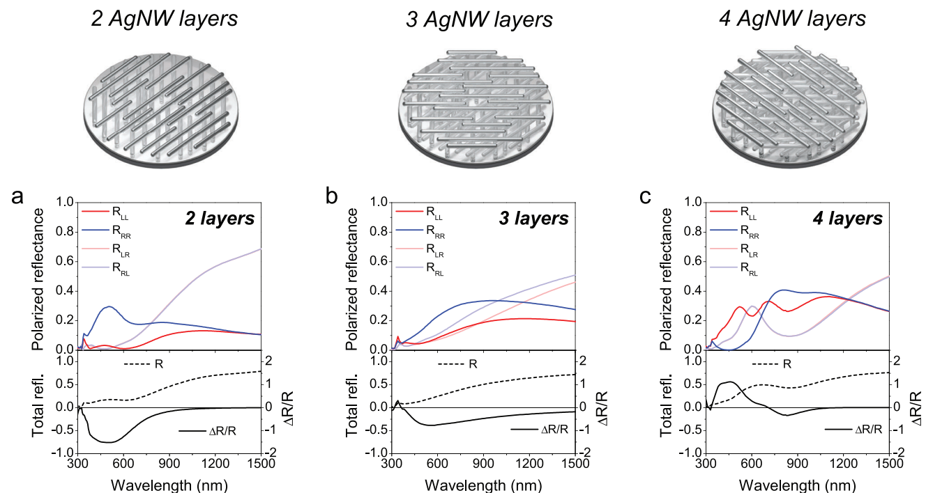
Figure 4. Spectra of the measured reflectance R labeled as function of the incoming and outgoing polarization states R_{i\sigma} and of the average reflectance R and the differential reflectance \frac{\Delta R}{R} for samples consisting of a varying number of layers of oriented AgNWs deposited on top of a silver mirror. The AgNW layers are oriented at +45^\circ (left-handed structure) and separated by a constant spacing of 13 nm. The sample consist of a) 2, b) 3, and c) 4 AgNW layers. Note that the sample in (a) is the same as the one of Figure 2b and Figure 3b.
