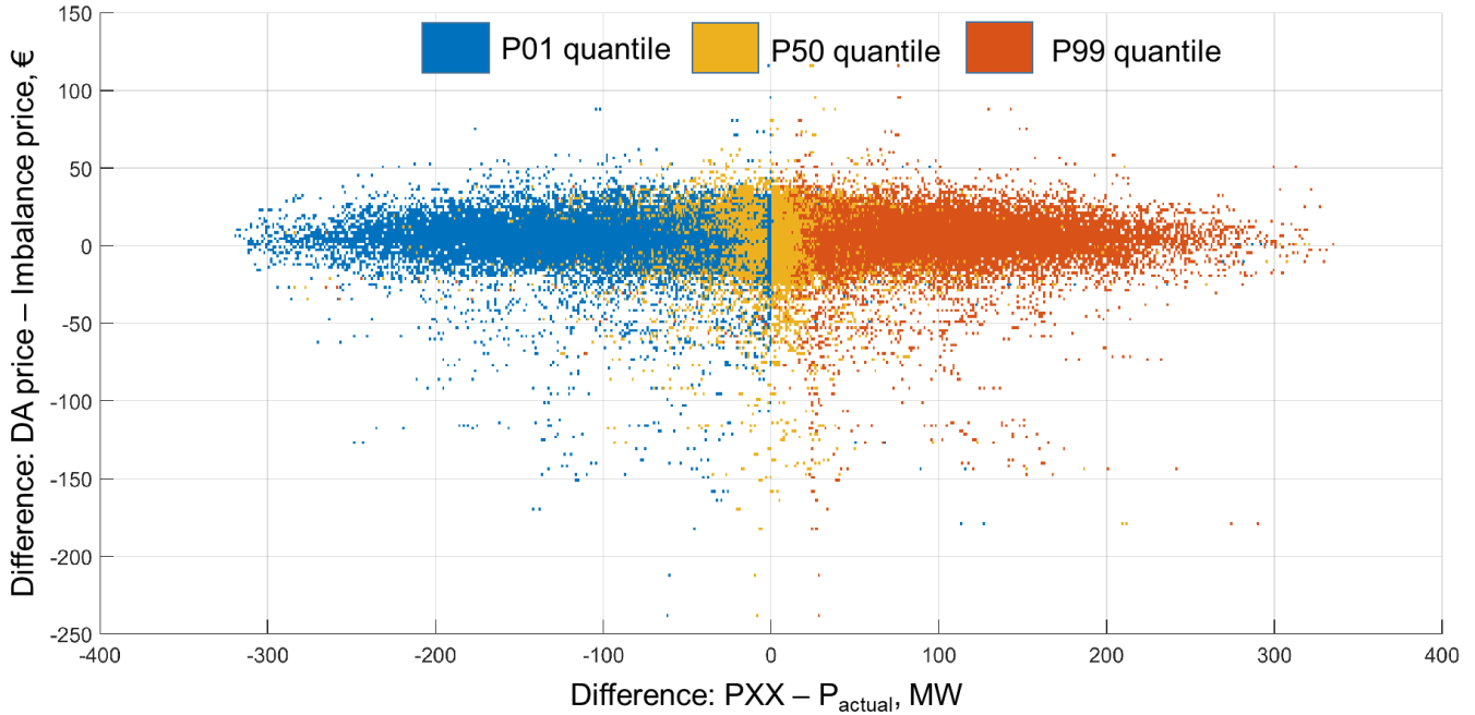
Figure 12 Scatter plot showing the price and power differences for a non-overplanted OWF
