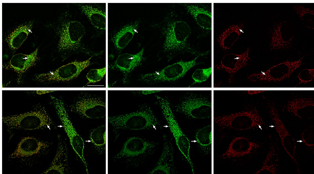
Figure 4. Colocalization studies of Cyn 7 and Ru-Cyn-1 with Mitotracker Green. Optical section of HeLa cells treated for 1 h at 37 °C with 10 \mu\text{M} Cyn 7 (top) and 10 \mu\text{M} Ru-Cyn-1 (bottom) and 30 min with MTG. Left: merged images; center: MTG signal; right: compound signal. Arrows point out some colocalizing mitochondria. Scale bar = 20 \mu\text{m} .
