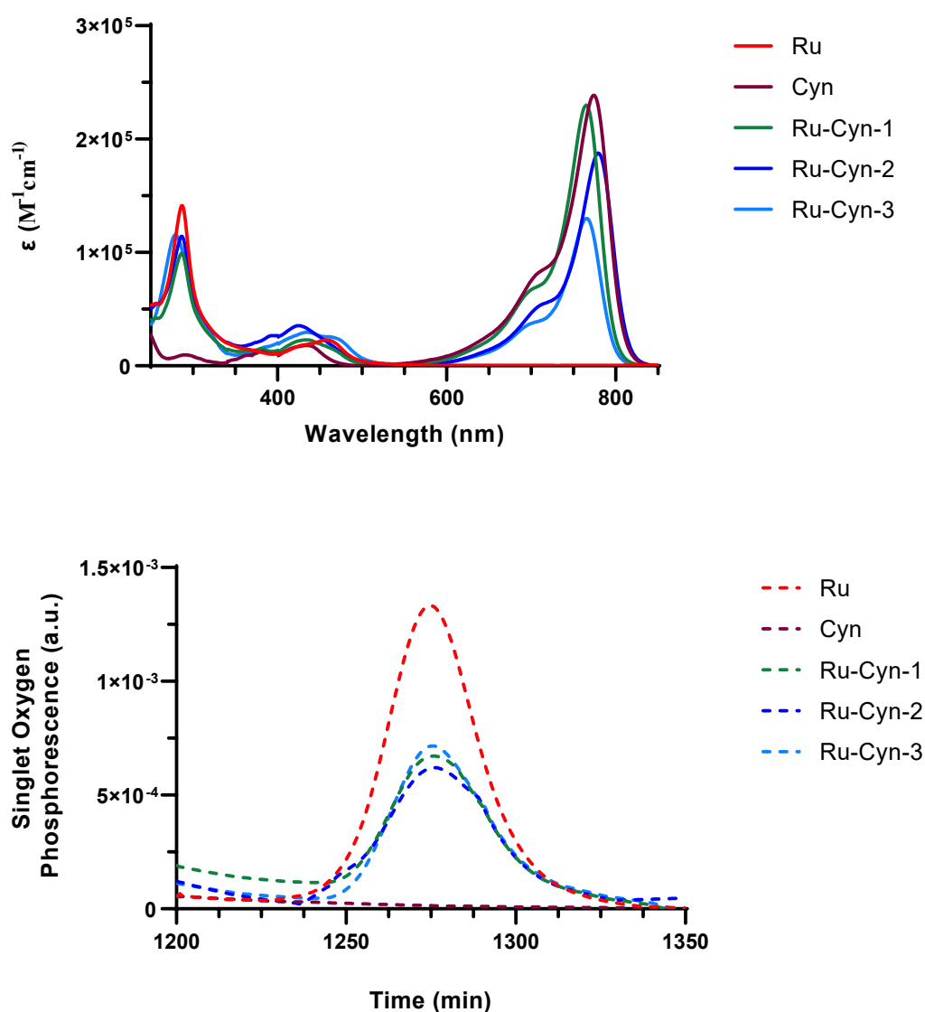
Figure 2. UV-Vis absorption spectra (Top) and singlet oxygen ( ^1O_2 ) emission spectra ( \lambda_{ex} = 450 nm) (Bottom) of the compounds measured in acetonitrile.
