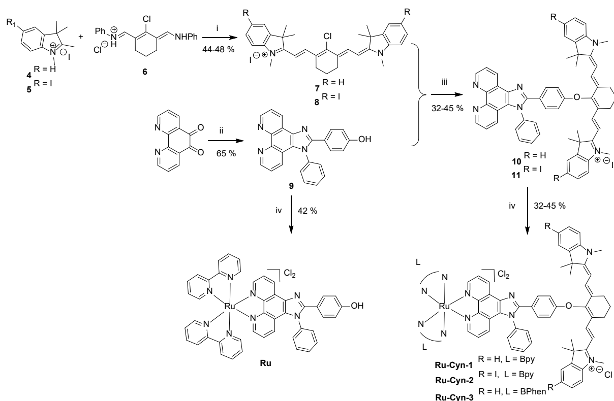
Scheme 1. Synthetic route for the preparation of Ru-Cyn-1-3 and Ru : (i) NaOAc, EtOH, 60 °C, 4 h; (ii) 4-hydroxybenzaldehyde, aniline, NH 4 OAc, AcOH, reflux, 15 h; (iii) NaH, DMF, 25 °C, 24 h; (iv) [Ru(Bpy) 2 Cl 2 ] or [Ru(Bphen) 2 Cl 2 ], H 2 O/EtOH (1:1, v/v), 70 °C, 15 h.
