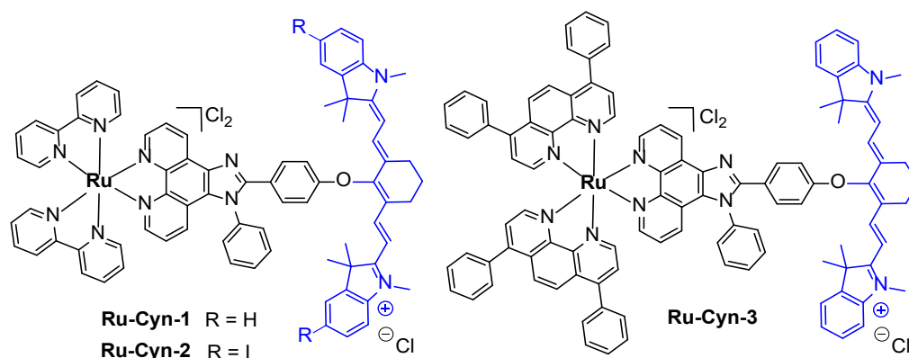
Figure 1. Structures of the ruthenium(II)-cyanine complexes ( Ru-Cyn-1-3 ) investigated in this work.
