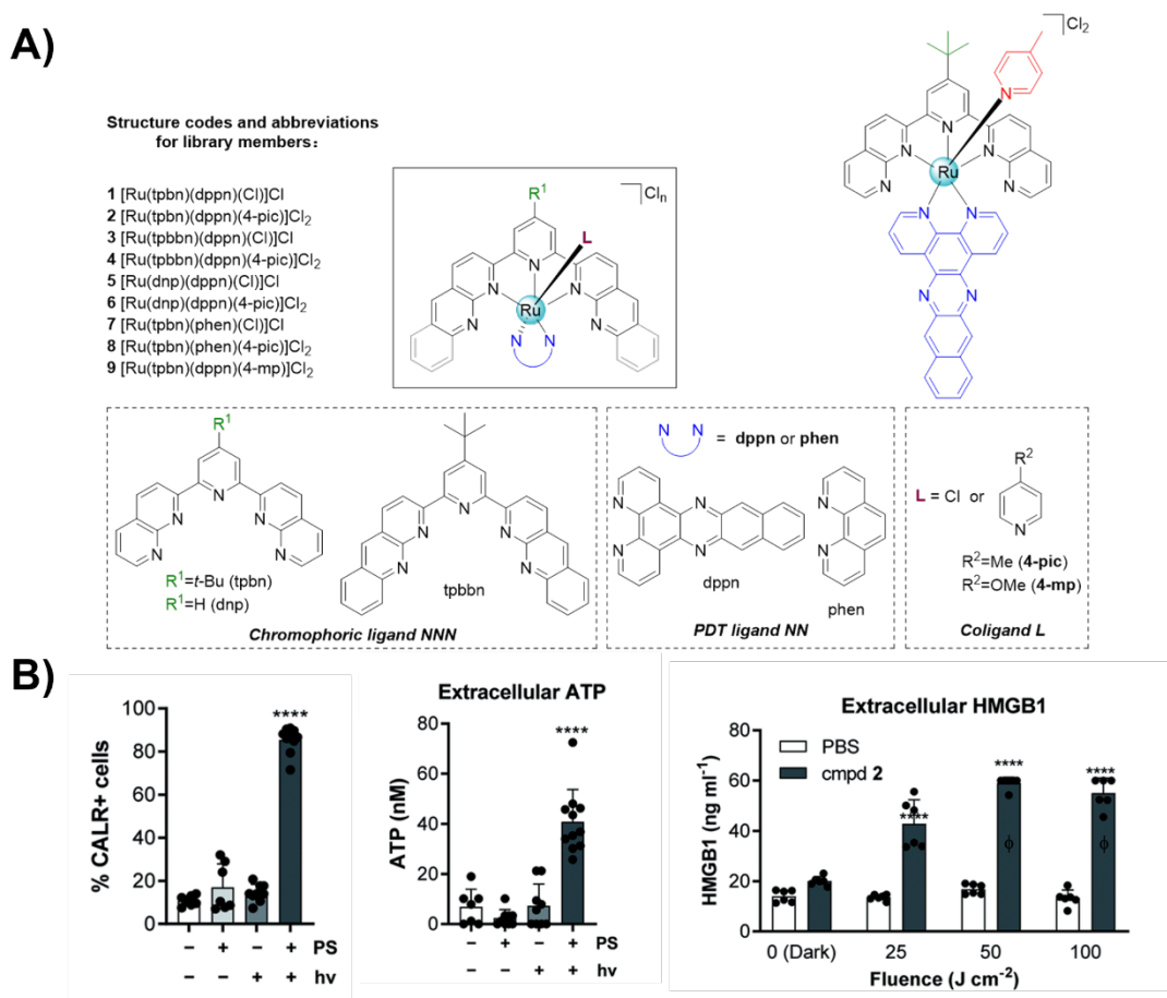
Fig. 7. (A) Discovery of Ru-based PSs that can induce ICD. (B) ICD-mediated biomarkers expression or release by 2-PDT. Reproduced with permission from Ref. 117. Copyright 2020 Royal Society of Chemistry
