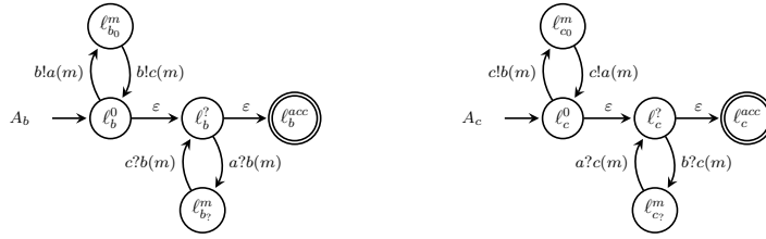
Figure 4: Sketch of A_b and A_c of \mathcal{S}_3 (only a single message m is considered).
