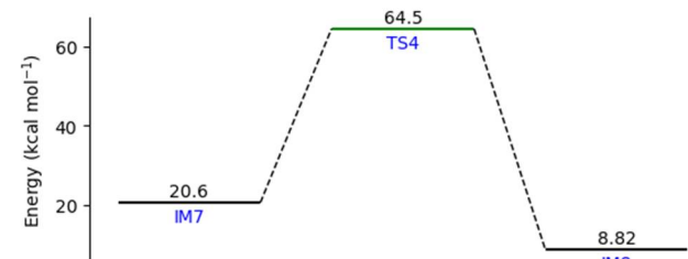
(c) Reaction 3
