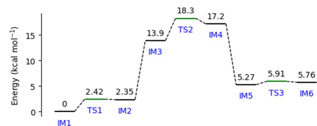
(b) Reaction 2
