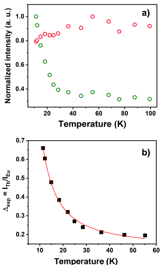
Figure 5. a) Temperature dependence of the normalized integrated area of I_{Tb} (green points) and I_{Eu} (red points) of Tb_{1.90}Eu_{0.10} -MOF upon 309 nm excitation, and b) Temperature-dependence of the thermometric parameter \Delta in the 10-55K range for the compound Tb_{1.90}Eu_{0.10} -MOF excited at 309 nm. The red line represents the calibration curve obtained by the best fit of the experimental points to the equation 1 ( r^2 > 0.99 ).
