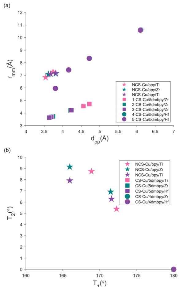
Figure 6. Summary of (a) d_{PP} , r_{mm} , (b) T_1 , and T_2 parameters for heterochiral \pi-\pi stacking interactions in the reported NCS compounds and compounds 1-5. The pink, green and purple squares and circles are eclipsed in (b).
