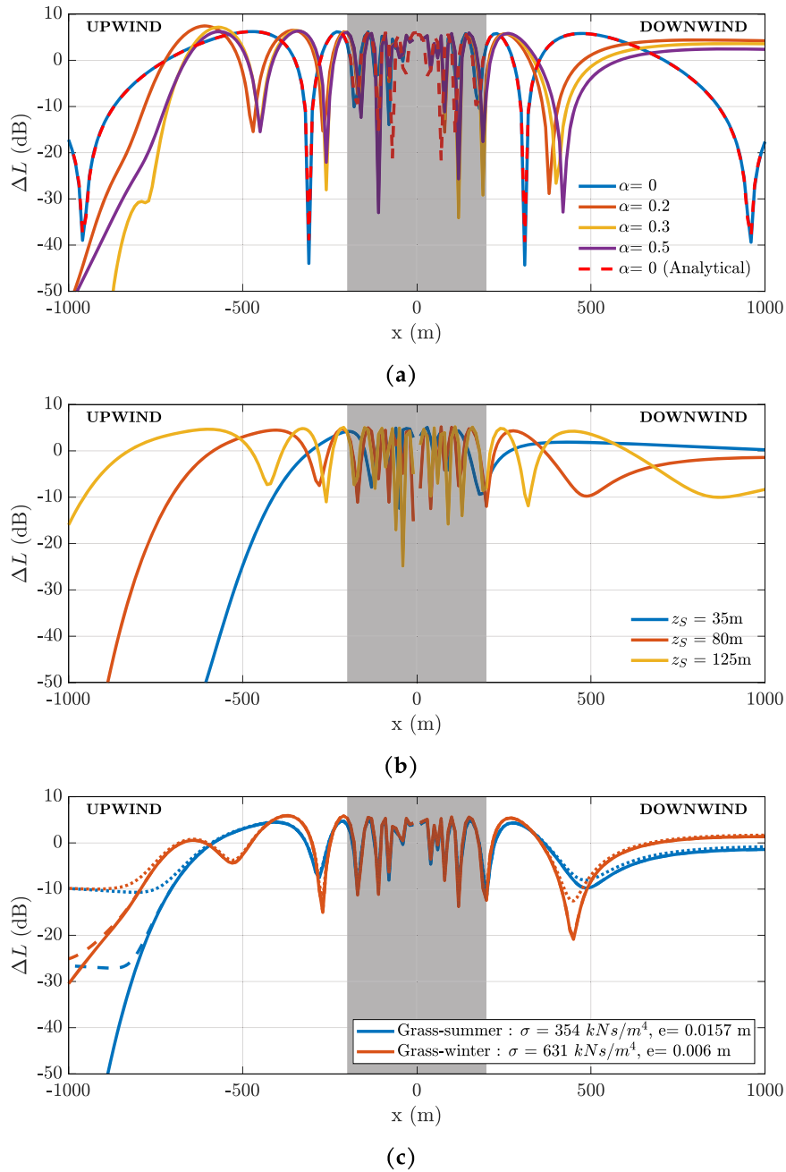
Figure 3. Relative SPL \Delta L calculated at f = 500 Hz for the receiver at height z_R = 2 m and x_R upwind ( -x ) and downwind ( +x ) with U_{ref} = 8 m/s at z_{ref} = 80 m for (a) different wind shear exponents \alpha with the source at z_S = 80 m and a hard ground with no turbulence in the atmosphere, (b) \alpha = 0.3 and with the grass ground in the summer and different source heights with no turbulence in the atmosphere, and (c) \alpha = 0.3 with the source at z_S = 80 m and different ground conditions and including turbulence in the atmosphere. The shaded area shows where the implemented WAPE-MM is not validated (solid line with no turbulence, dashed line with low turbulence and dotted line with strong turbulence).
