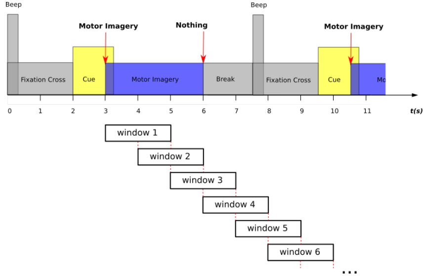
Figure 2: Figure explaining the introduction of the nothing event and the sliding windows in the BCI Dataset 2a (BNCI2014001) [11]. In this example, we use a window of 2 seconds with an overlapping of 50%
