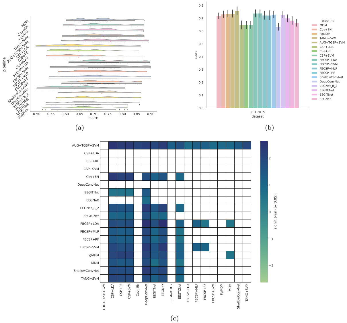
Figure 11: Result for BNCI2015001 classification, using Within-Session evaluation. Plot (a) shows the rain clouds plots for each pipeline, showing the distribution of the score of every subject. Plot (b) shows a bar plot of the score with the error of the different pipelines and for every datasets considered. Plot (c) shows the meta analysis of the different methods considered. This plots the significance that the algorithm on the y-axis is better than the one on the x-axis. The color represents the significance level of the difference of accuracy, in terms of t-values, and we show only the significant interactions ( p < 0.05 ).
