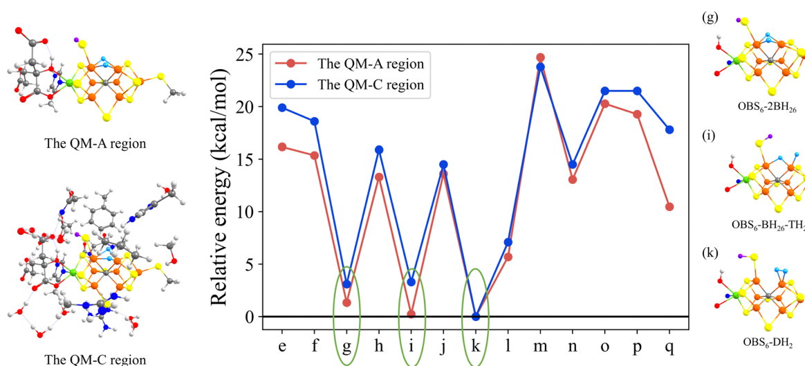
Fig. 4 The comparison of relative QM/MM energies using r^2\text{SCAN} for models ( e–q ) between using the QM-A and QM-C regions. The labels of the x-axis indicate the models defined in Fig. 2. QM-A region contains 59 atoms while QM-C contains 191 atoms. The spin states and BS solutions are the same as Fig. 2.
