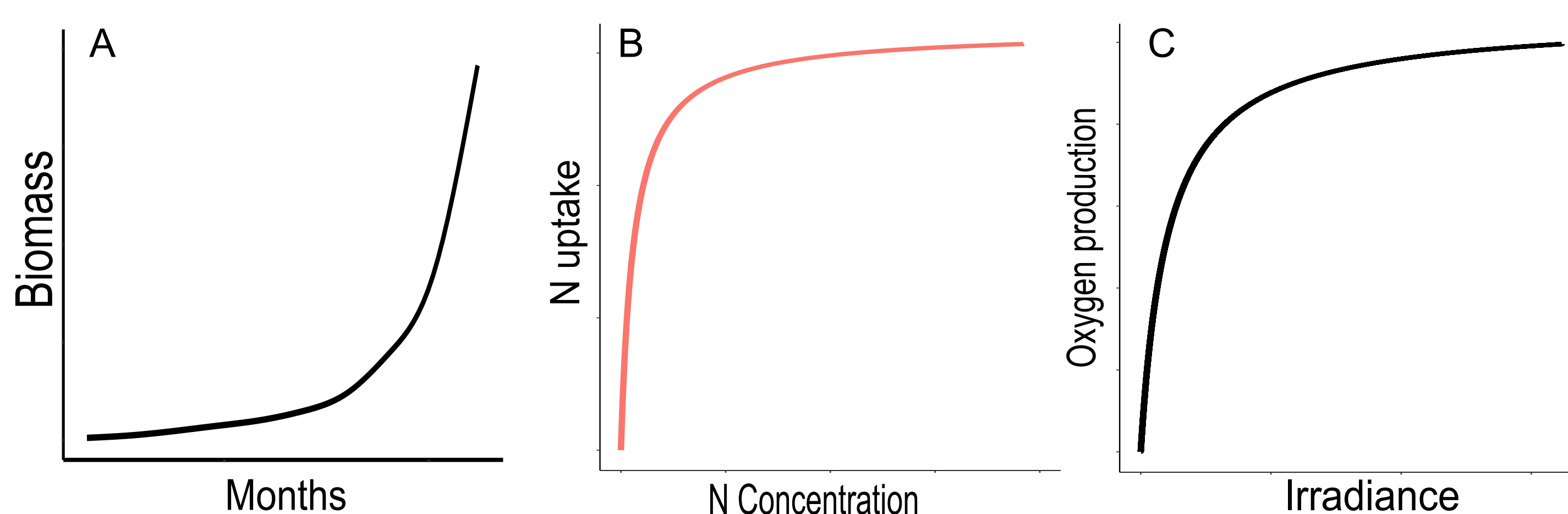
Figure 1. Simulations of A) Biomass evolution B) N uptake and C) Oxygen production. Adaptation of [10] GitHub code based on algae models previously developed [7, 10].
