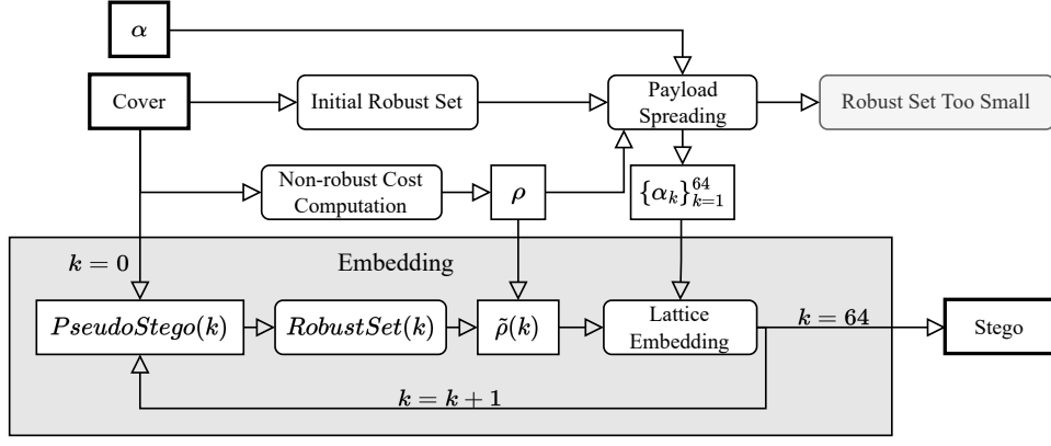
Fig. 3. Main steps of the embedding algorithm.
