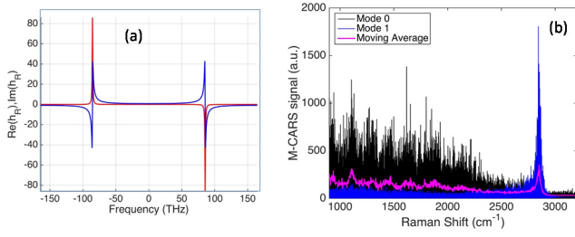
Fig. 7. M-CARS Simulation. (a) Representation of vibrational mode at 85.5 THz (2852 \text{cm}^{-1} ). (b) M-CARS spectrum produced by the four-wave mixing M-CARS process obtained from the bimodal excitation of the microstructured fiber.
