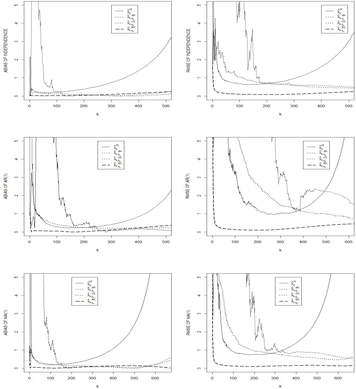
FIGURE 4.2 – Simulation of the extreme quantiles estimators : By row, Models 1, 2, 3. By column, ABias ( left ) and RMSE ( right ) as functions of k .
