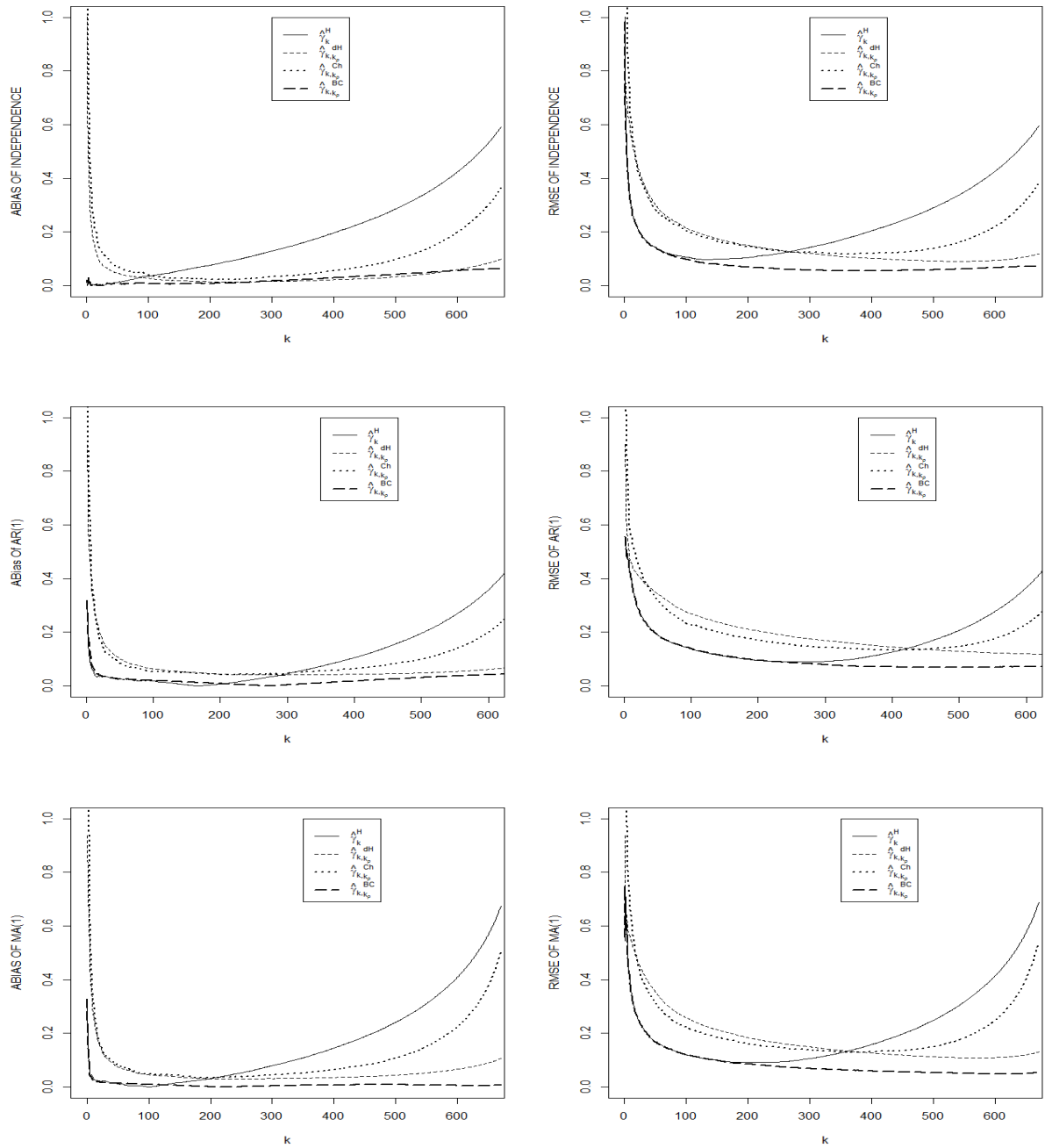
FIGURE 4.1 – Simulation of the tail index : By row, Models 1, 2, 3. By column, ABias ( left ) and RMSE ( right ) as functions of k .
