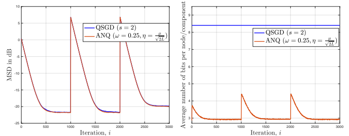
Fig. 7. Network performance in non-stationary environment (i.e., the solution \mathcal{W}^o in (3) is changing over time due to changes in the individual costs \{J_k(w_k)\} ) when the probabilistic ANQ quantizer of Example 2 and the QSGD quantizer of Table I are used. (Left) Evolution of the MSD learning curves. (Right) Evolution of the average number of bits per node, per component. The variable-rate scheme described in Sec. II-A is used in the probabilistic ANQ case.
