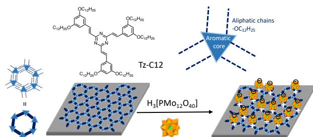
Scheme 1. The Tz-C12 molecule and the strategy of deposition of oxo-clusters on self-assembled Tz-C12 on HOPG in a honeycomb arrangement.
