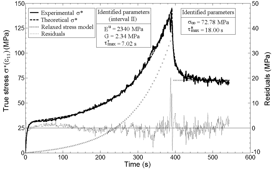
Figure 9: Tensile test followed by a relaxation for specimen B. Experimental data, fitted curve (Eq. 15) and residuals plotted as a function of time. Identified parameters are E^u , G , \tau_{\max}^T , \sigma_{\infty} and \tau_{\max}^R - Strain rate of 5 \times 10^{-3} \text{ s}^{-1} (400 s correspond to a true strain of 2).
