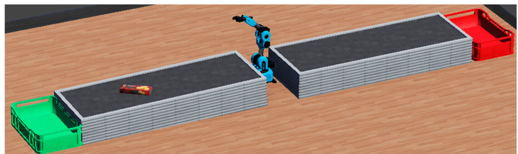
Figure 11. The cobot received the MQTT message «RIGHT» for the topic «bci_team/arm». Accordingly, the packet is send to the conveyor belt situated on its right.
